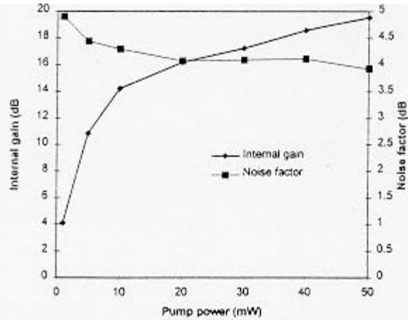
Fig. 6. Variations of internal gain and noise factor with pump power for the waveguide with optimum length (6 mm), signal ( \lambda_{\text{sig}} = 1.530 \mu\text{m} ) and pump wavelengths ( \lambda_{\text{pump}} = 1.000 \mu\text{m} ).
