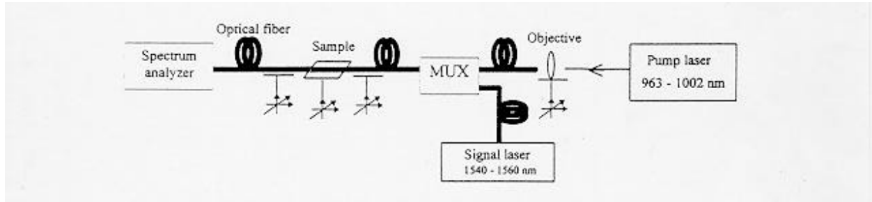
Fig. 1: Schematics of gain measurement setup.
